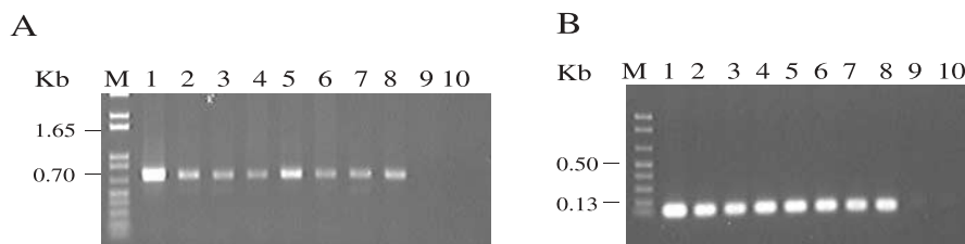
Figure 2. Molecular characterization of putative transformants via PCR. A: Amplification of a specific 700-bp fragment from the \beta -glucuronidase ( GUS ) gene (A). B: 130-bp fragment amplified from the neomycin phosphotransferase ( NPTII ) gene. M: Molecular weight marker (1 kb plus DNA ladder). Lanes labeled 1-9 contained the following templates in the PCR reaction mixtures: p35S-GUS-INT (positive control); genomic DNA from 7 separate transformation events (lines); and a nontransformed plant (negative control), respectively. Lane 10 was no-template (double-distilled H 2 O) control.
