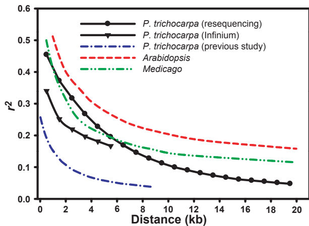
Fig. 4 Genome-wide linkage disequilibrium (LD) in Populus trichocarpa based on common single-nucleotide polymorphisms (SNPs) (i.e. minor allele frequency (MAF) \geq c. 0.10 ). Black circles and triangles correspond to average values of r^2 for interlocus distances grouped in 1-kb bins based on analyses of genome resequencing ( n = 16 trees, MAF \geq 0.094 ) and analyses of Infinium SNP data for 3704 candidate genes ( n = 120 trees, MAF \geq 0.10 ), respectively. Data from a previous small-scale study in P. trichocarpa (Wegrzyn et al. , 2010) and for the primarily self-pollinating plants Arabidopsis thaliana (Kim et al. , 2007) and Medicago truncatula (Branca et al. , 2011) are illustrated using dashed and/or dotted lines.
