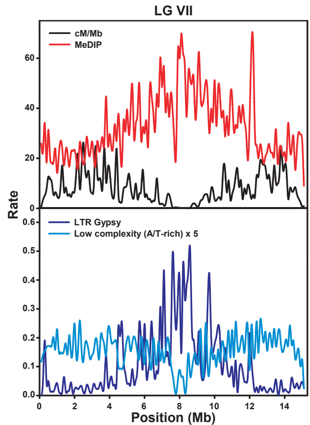
Fig. 7 Correlates of recombination in Populus trichocarpa . Chromosome-wide patterns of variation of: recombination rates (cM/Mb) estimated from linkage disequilibrium (LD); relative degree of methylation (methylated DNA immunoprecipitation, MeDIP), measured as the number of MeDIP reads per kilobase of target sequence per million reads mapped (Supporting Information Methods S2); the proportion of bases in long terminal repeat (LTR) Gypsy retrotransposons; and the proportion of bases in A-, T- or AT-rich low-complexity sequences (multiplied by five to equalize scales). All data are summarized in 100-kb windows. Values of 4N_e c were converted to recombination frequencies (cM/Mb) using the LD-based estimate of N_e for Linkage Group VII (Fig. S4).
