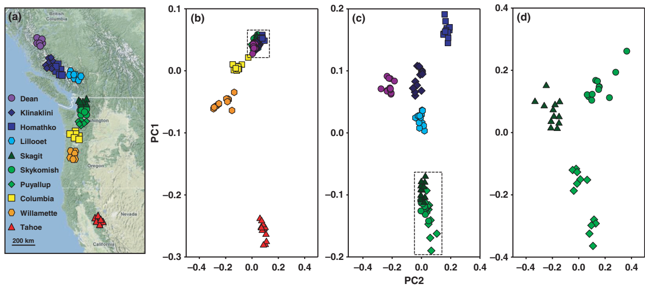
Fig. 2 Population structure in Populus trichocarpa based on Infinium single-nucleotide polymorphism (SNP) data. (a) Sampling locations of 120 P. trichocarpa trees from 10 subpopulations chosen to span the geographic distribution of the 16 resequenced trees. (b–d) Major axes of variation based on principal component analysis (PCA) of 22 280 SNPs on a range-wide scale (b), after excluding trees from the clearly differentiated Tahoe, Willamette and Columbia subpopulations (c), and within the most homogeneous set of subpopulations in western Washington (d). Clusters which include trees from multiple subpopulations (dotted frames in b and c) were re-analyzed at finer spatial scales after excluding clearly differentiated trees.
