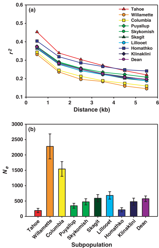
Fig. 6 Variation of linkage disequilibrium (LD; r^2 ) and LD-based estimates of effective population size ( N_e ) across 10 subpopulations of Populus trichocarpa . (a) Average values of r^2 for interlocus distances grouped in 1-kb bins based on analyses of Infinium single-nucleotide polymorphism (SNP) data (minor allele frequency (MAF) \geq 0.10 ) for 12 trees in each subpopulation. (b) Estimates of N_e based on relating estimates of the scaled recombination rate ( 4N_e c ) from the Infinium SNP data to direct estimates of recombination from a dense SNP linkage map. Subpopulations are ordered by latitude from south (left) to north (right).
