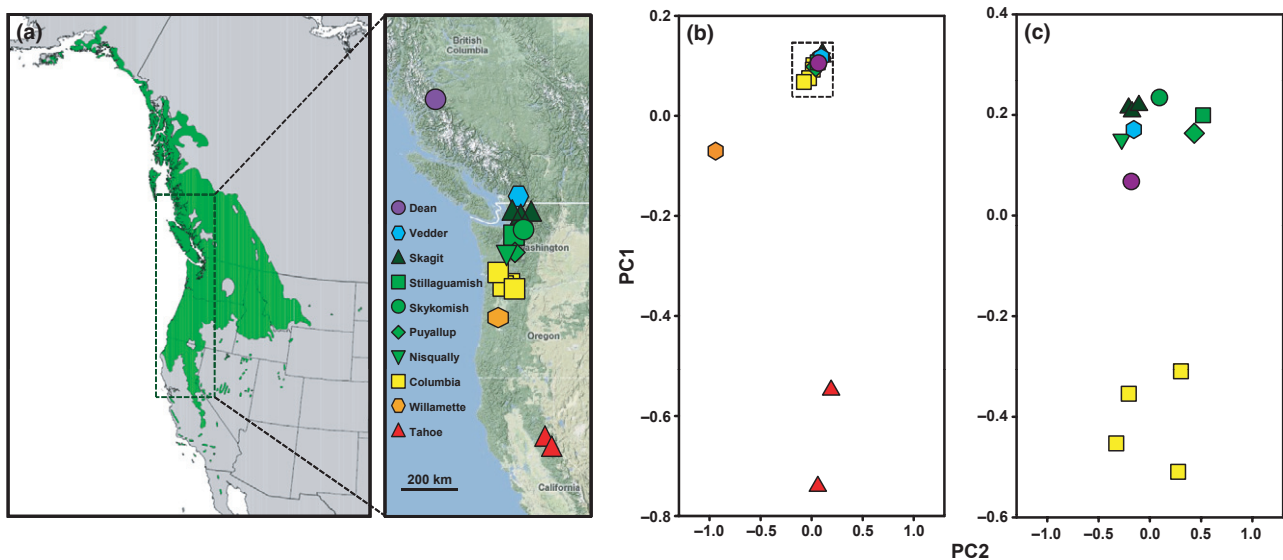
Fig. 1 Population structure in Populus trichocarpa based on genome resequencing data. (a) Sampling locations of the 16 P. trichocarpa trees that were resequenced, relative to the species range (Little, 1971). (b, c) Major axes of variation based on principal component analysis (PCA) of 235 259 single-nucleotide polymorphisms (SNPs) on a range-wide scale (b) and after excluding the clearly differentiated Tahoe and Willamette trees (c). The cluster which includes trees from multiple locations (dotted frame in b) was re-analyzed at a finer spatial scale (c).
