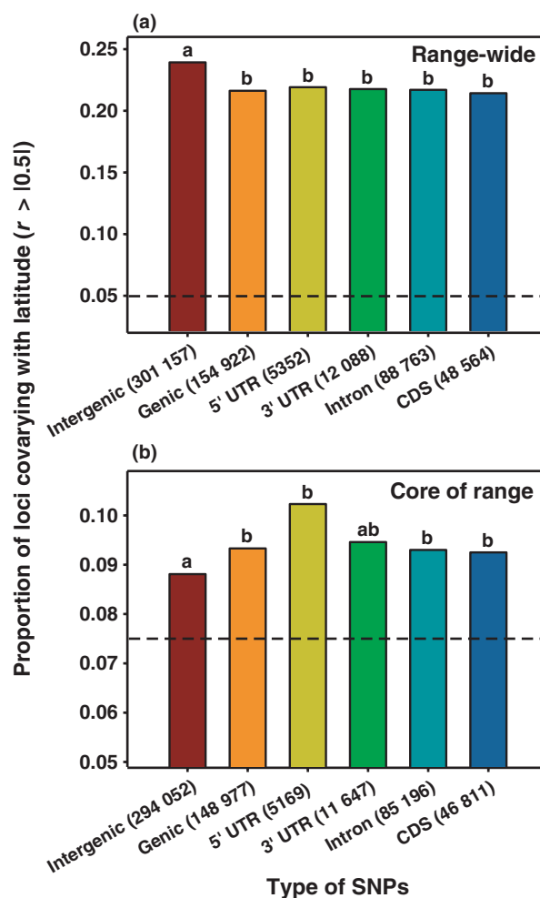
Fig. 3 Latitudinal allele frequency gradients in Populus trichocarpa based on genome resequencing data. Proportions of single-nucleotide polymorphisms (SNPs) that covary moderately or strongly with latitude (i.e. Pearson's |r| > 0.50 ). (a) 456 079 SNPs that passed Hardy–Weinberg equilibrium (HWE) filtering based on data for all trees ( n = 16 ). (b) 443 029 SNPs that passed HWE filtering based on data for 13 trees, excluding the strongly differentiated trees sampled from the Tahoe and Willamette subpopulations (Figs 1, 2). In each graph, bars annotated with different letters correspond to significantly different proportions ( P < 0.002 based on contingency table \chi^2 tests). Dashed lines indicate the proportions of SNPs expected to covary with latitude (i.e. |r| > 0.50 ) based on 1000 permutations of SNP genotypes and source latitudes. The number of loci in each category is shown in parentheses. CDS, coding DNA sequence; UTR, untranslated region.
