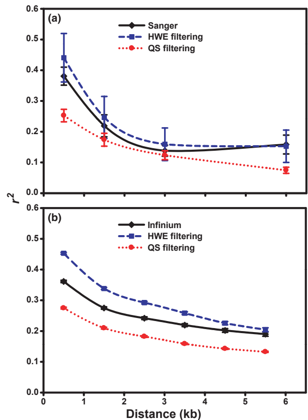
Fig. 5 Effect of filtering criteria on estimates of linkage disequilibrium (LD; r^2 ) based on genome resequencing data relative to estimates based on Sanger resequencing data (a) and Infinium single-nucleotide polymorphism (SNP) data (b). All estimates are based on data for trees from the core of the range of Populus trichocarpa (i.e. excluding the strongly differentiated trees from the Tahoe and Willamette subpopulations). Error bars correspond to 95% confidence intervals based on 1000 bootstrap samples. (a) Average values of r^2 for SNPs located inside or within 2 kb of 10 candidate genes resequenced using Sanger technology (Table S2, n = 40 trees, minor allele frequency (MAF) \geq 0.10 , 1243 SNP pairs) and based on SNPs from the same regions that were genotyped by genome resequencing ( n = 13 trees, MAF \geq 0.115 ) and filtered using the Hardy–Weinberg equilibrium (HWE; 304 SNP pairs) and Quality Score (QS; 3760 SNP pairs) sets of criteria (Table 1). Pairwise r^2 values were grouped into 0–1, 1–2, 2–4 and 4–8 kb distance classes to ensure that each class contained at least 50 values in each dataset. (b) Average values of r^2 in 1-kb distance classes for loci inside or within 2 kb of 3704 candidate genes represented on the Infinium genotyping array ( n = 96 trees, MAF \geq 0.10 , 99 025 SNP pairs) and based on SNPs from the same regions that were genotyped by genome resequencing ( n = 13 trees, MAF \geq 0.115 ) and filtered using the HWE (170 186 SNP pairs) and QS (1 801 953 SNP pairs) sets of criteria.
